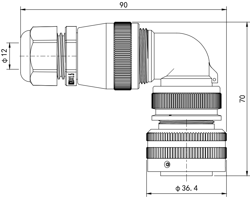
弯式插头 Curved plug
