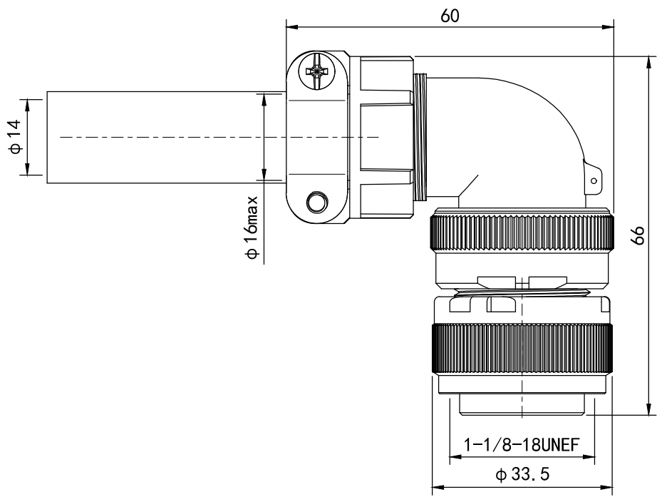
弯式插头 Curved plug
