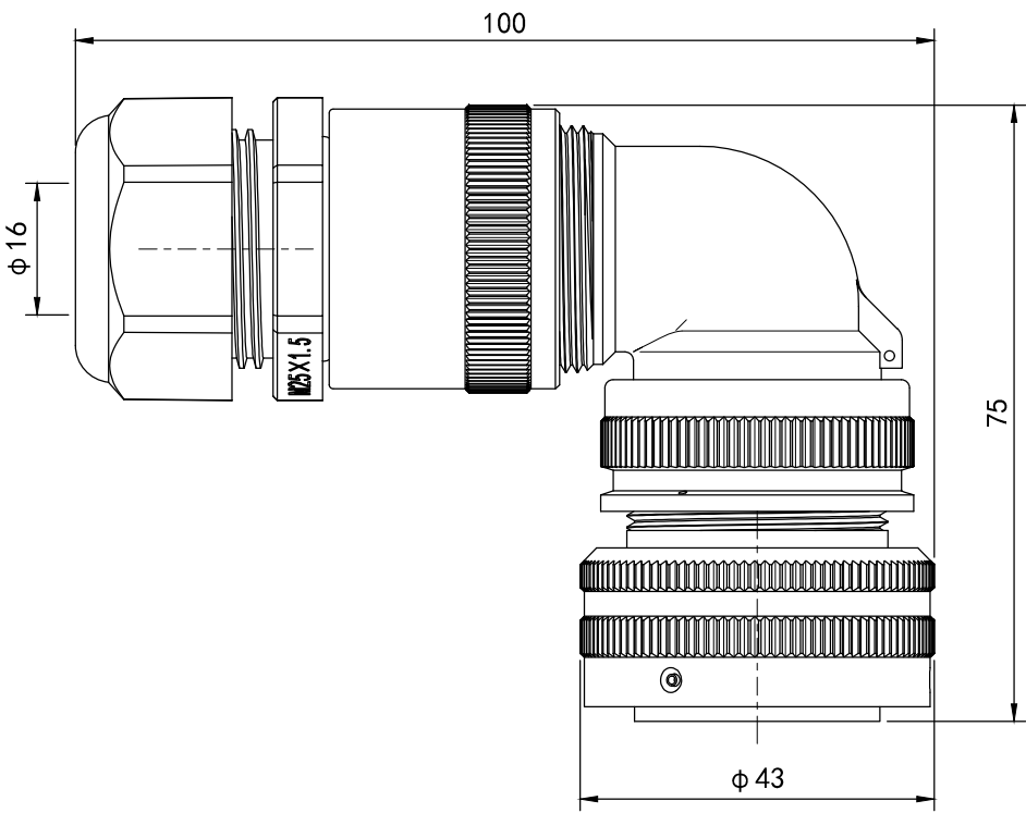
弯式插头 Curved plug
