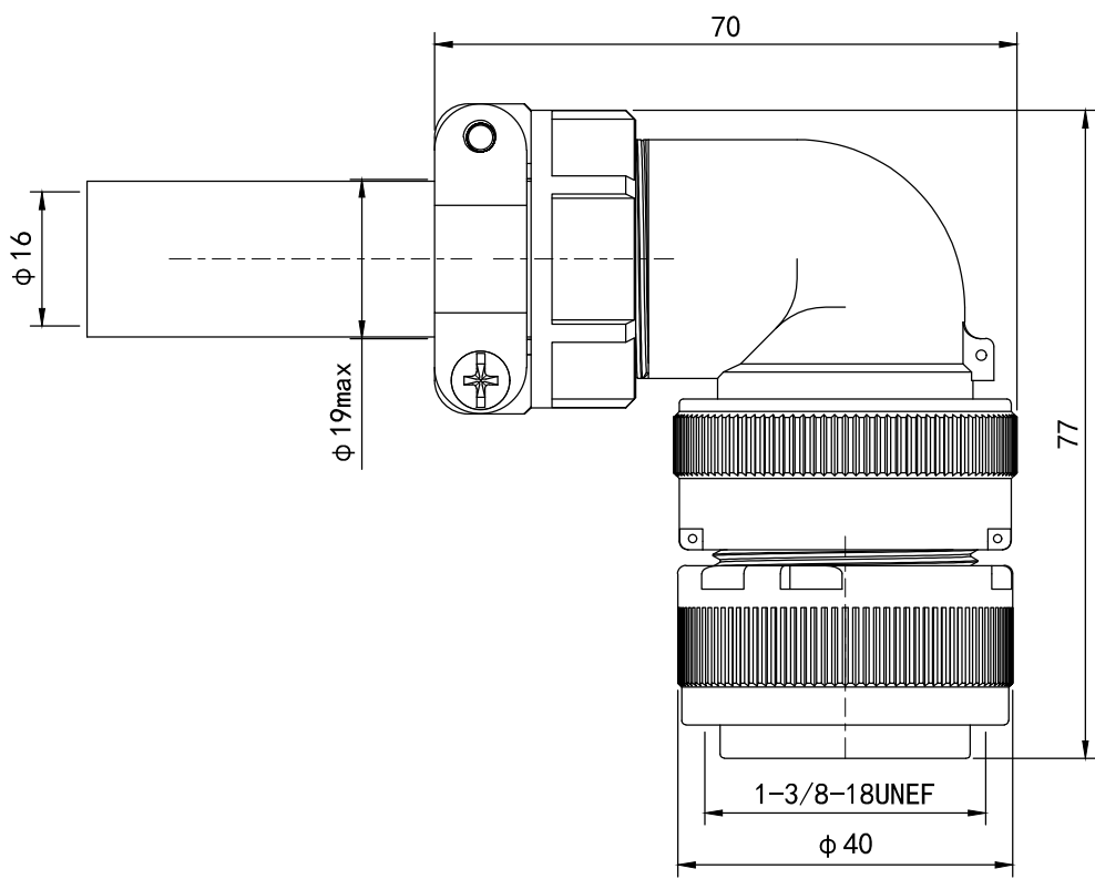
弯式插头 Curved plug
