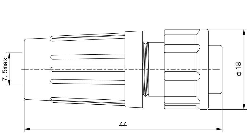
直式卡扣插头 Straight buckle plug
