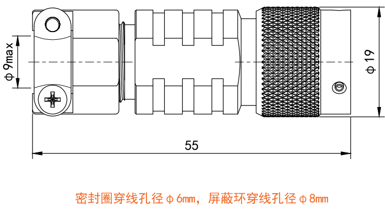
直式卡扣插头 Straight buckle plug
