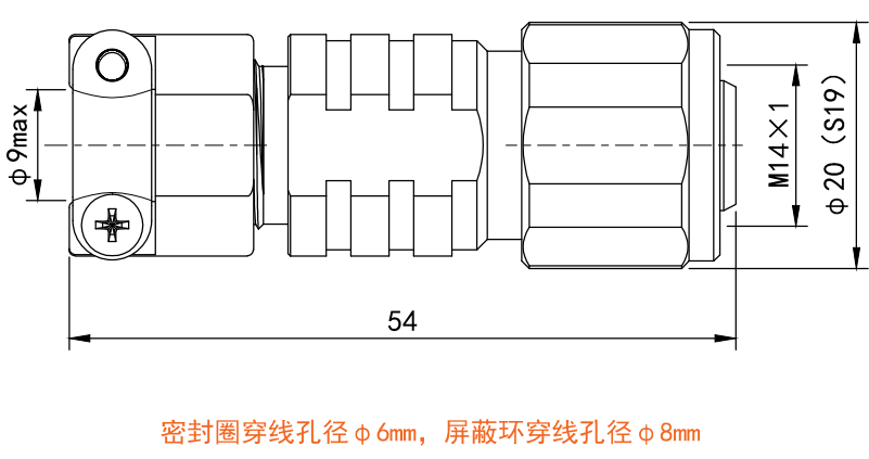
直式卡扣插头 Straight buckle plug
