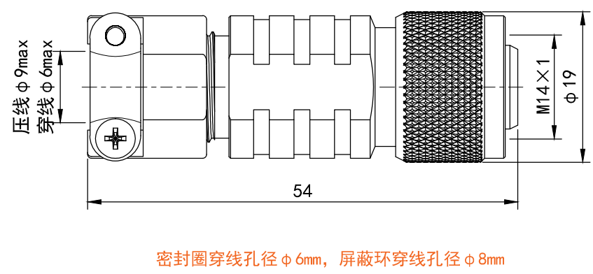
B型直式螺纹插头 B-type straight thread plug
